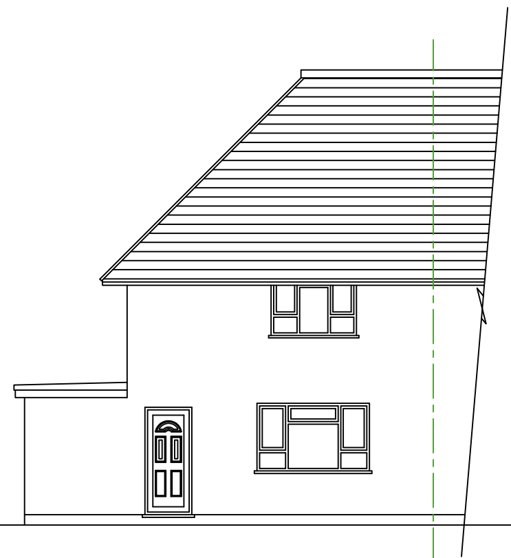
Existing SEE Elevation
