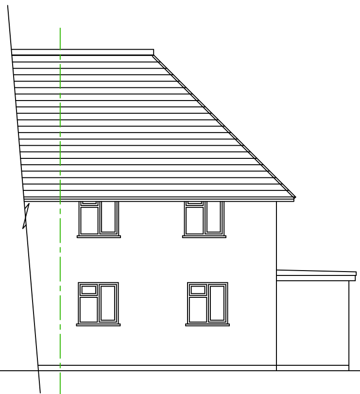
Existing NNW Elevation
