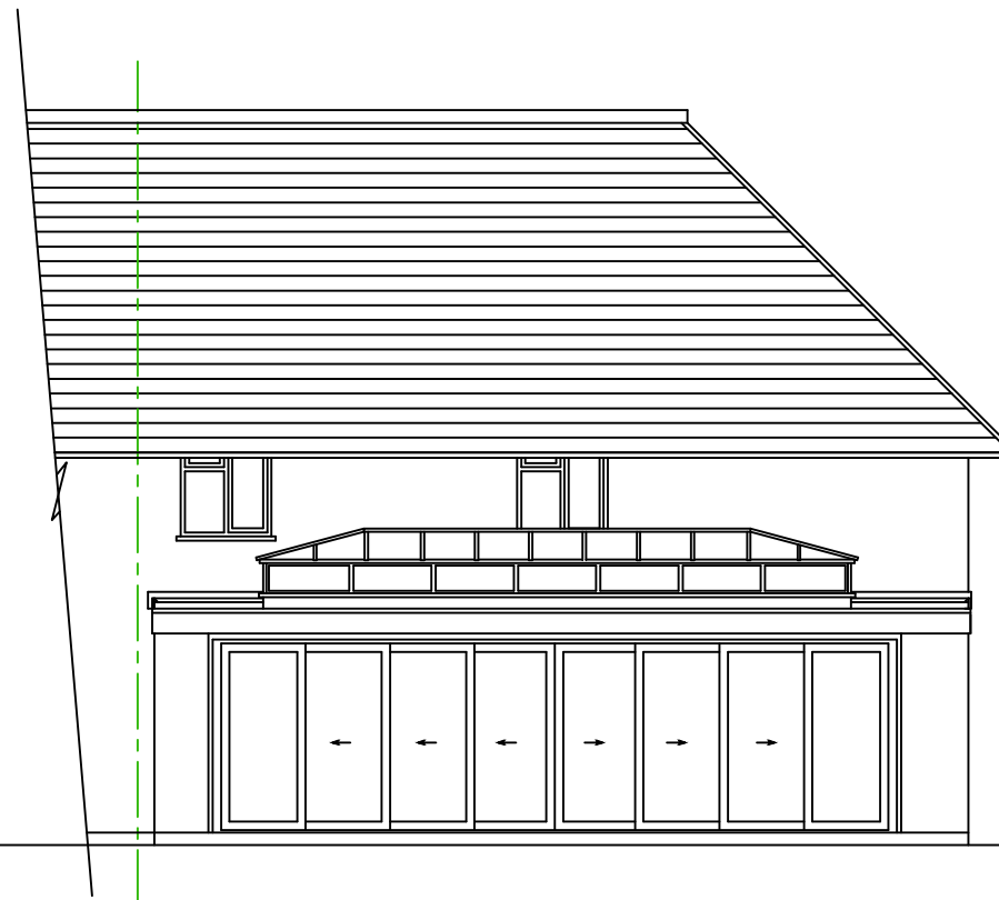
Proposed NNW Elevation
