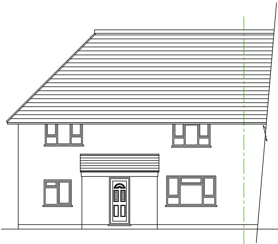
Proposed SEE Elevation
