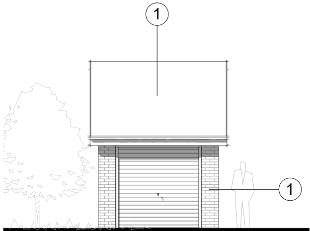
Front Elevation 1 : 100
