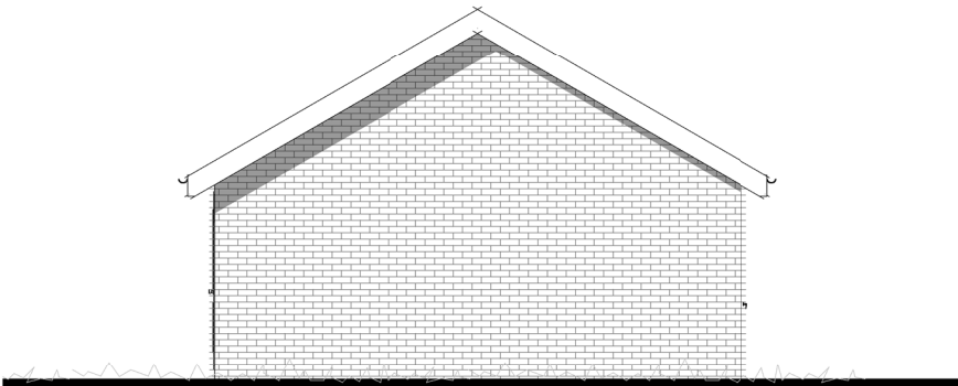
Side Elevation B 1 : 100
