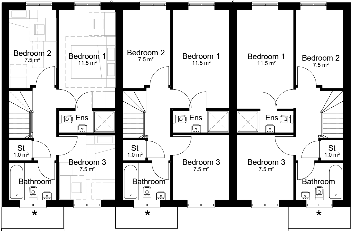
Level 01-First Floor (Plots 005-013/176-178) 1 : 100
