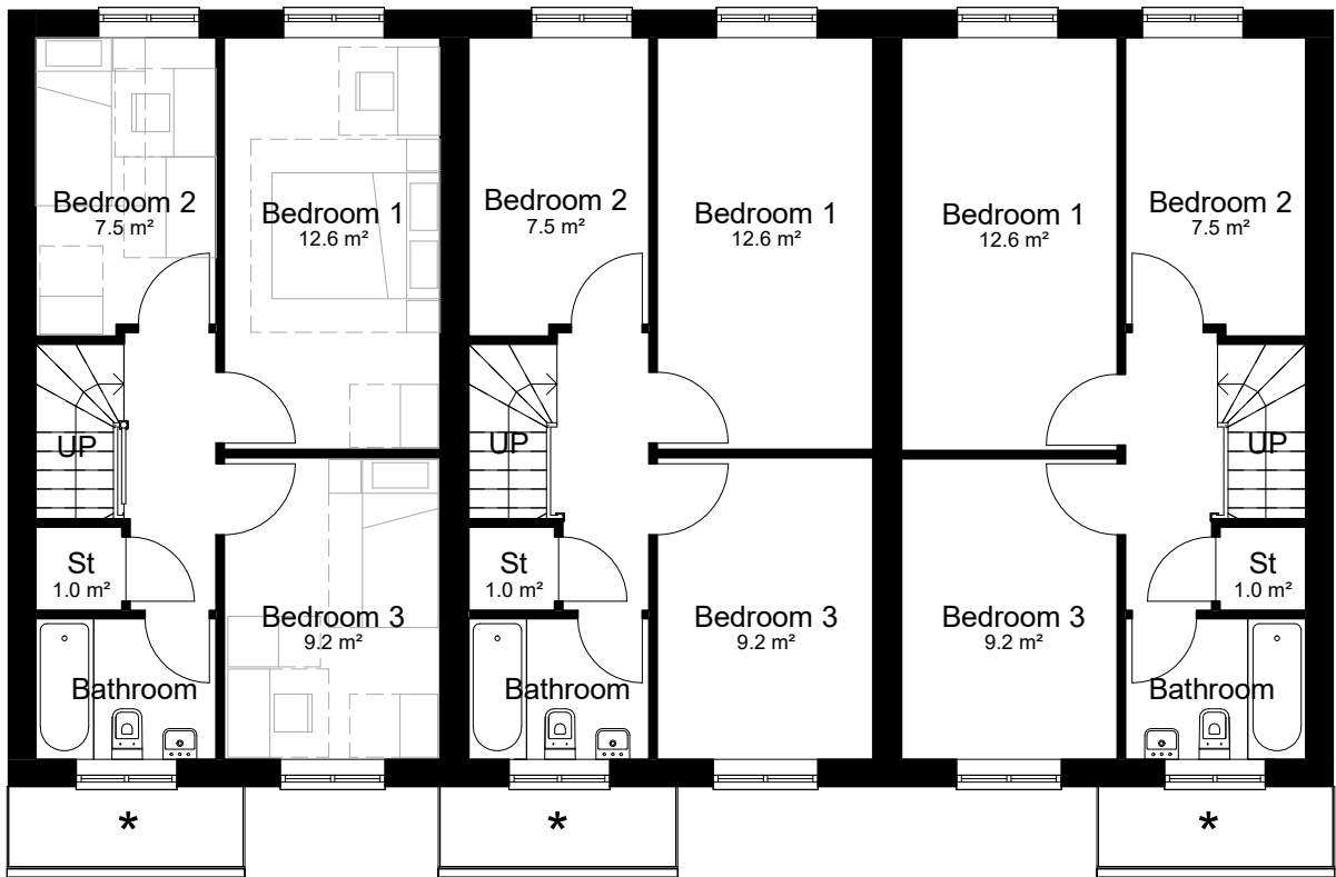
Level 01-First Floor (Plots 167-169) 1 : 100
