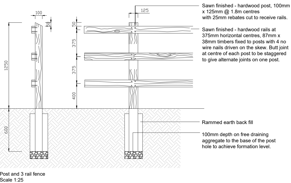
Post and 3 rail fence Scale 1:25
