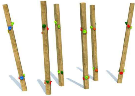
1. Traversing Trees
