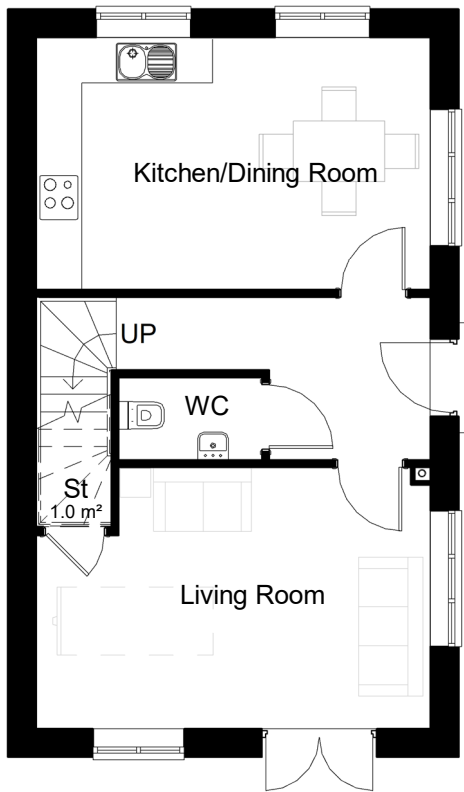
Level 00-Ground Floor 1 : 100
