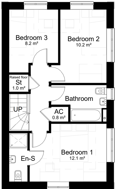
Level 01-First Floor 1 : 100
