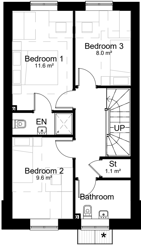
Level 01-First Floor 1 : 100
