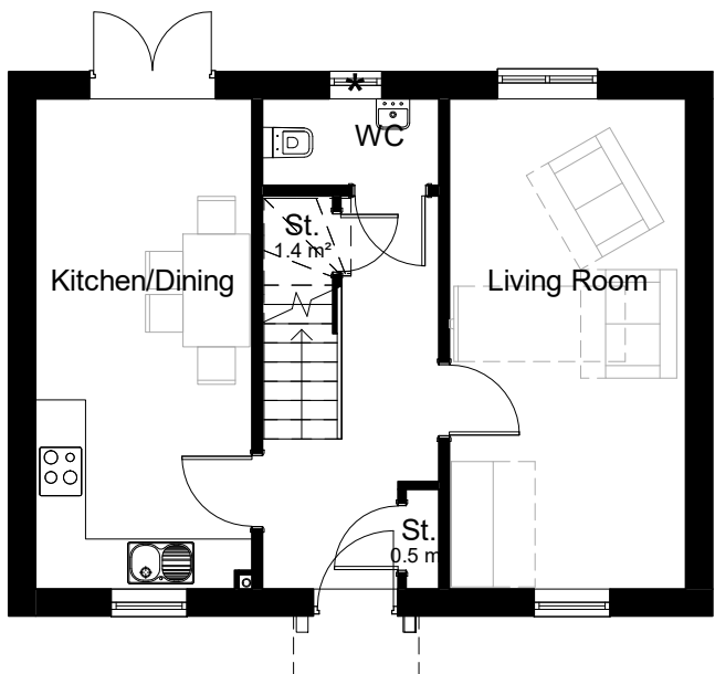
Level 00-Ground Floor 1 : 100
