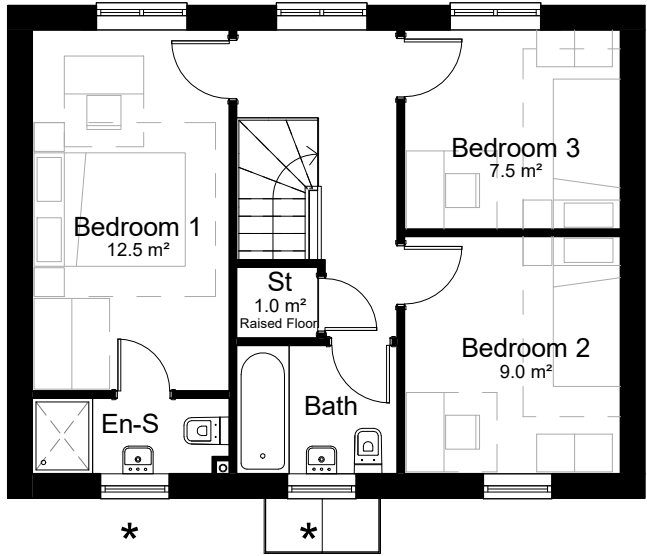
Level 01-First Floor 1 : 100
