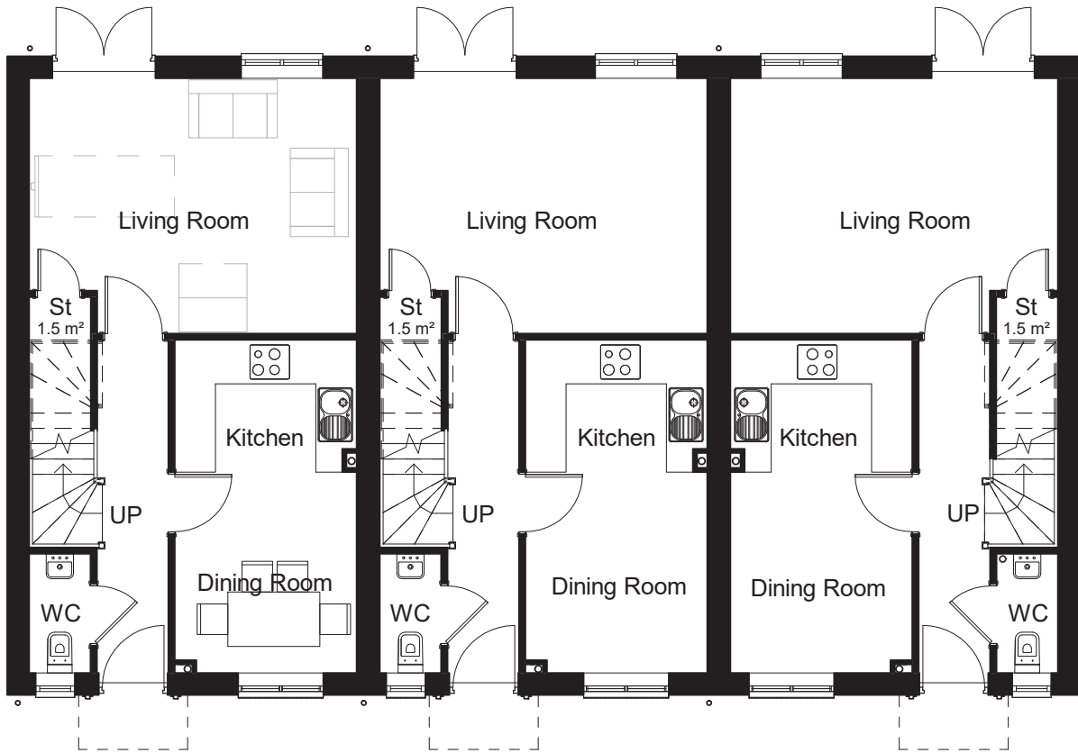
Level 00-Ground Floor 1 : 100
