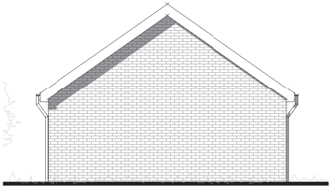
Side Elevation A 1 : 100
