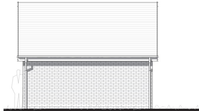
Rear Elevation 1 : 100
