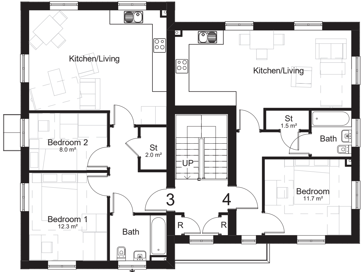
Level 01-First Floor 1 : 100
