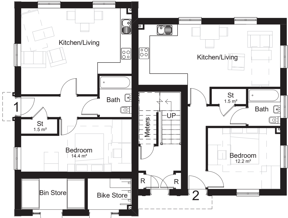
Level 00-Ground Floor 1 : 100
