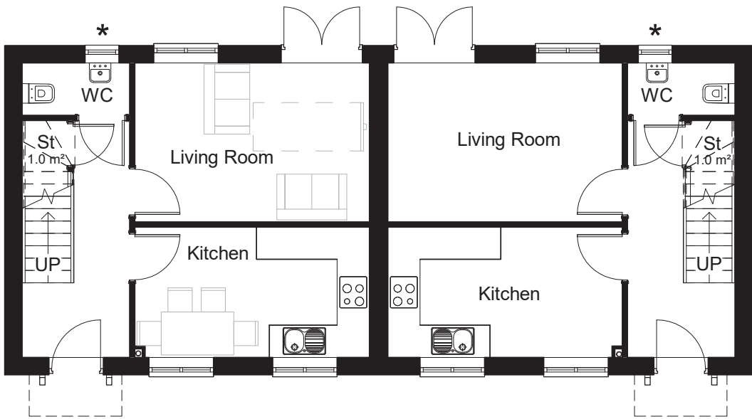
Level 00-Ground Floor 1 : 100
