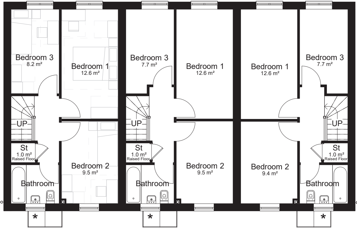
Level 01-First Floor (Plots 269-271) 1 : 100
