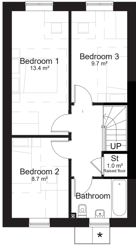
Level 01-First Floor 1 : 100
