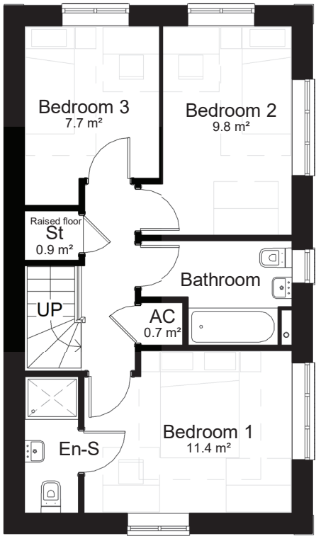
Level 01-First Floor 1 : 100
