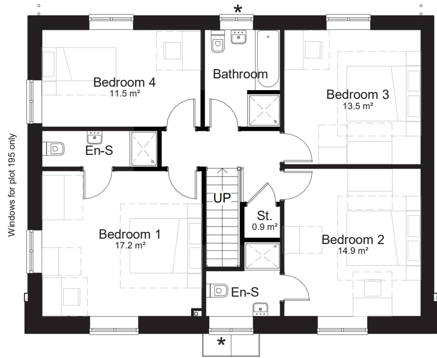
Level 01-First Floor 1 : 100
