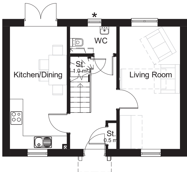
Level 00-Ground Floor 1 : 100
