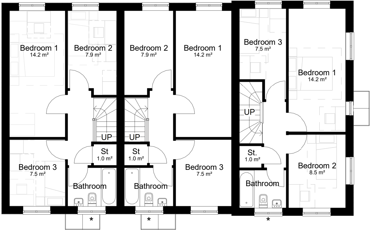
Level 01-First Floor (Plots 361-363) 1 : 100
