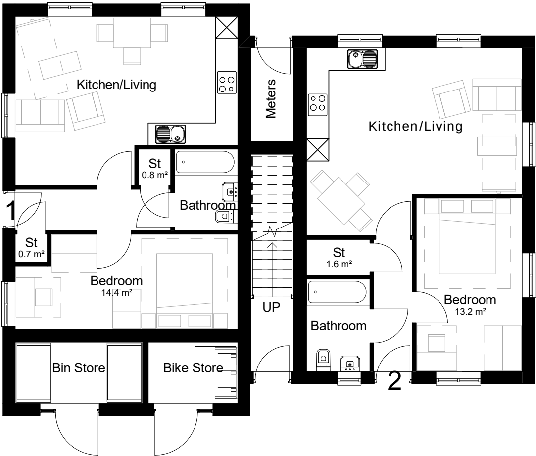
Level 00-Ground Floor 1 : 100
