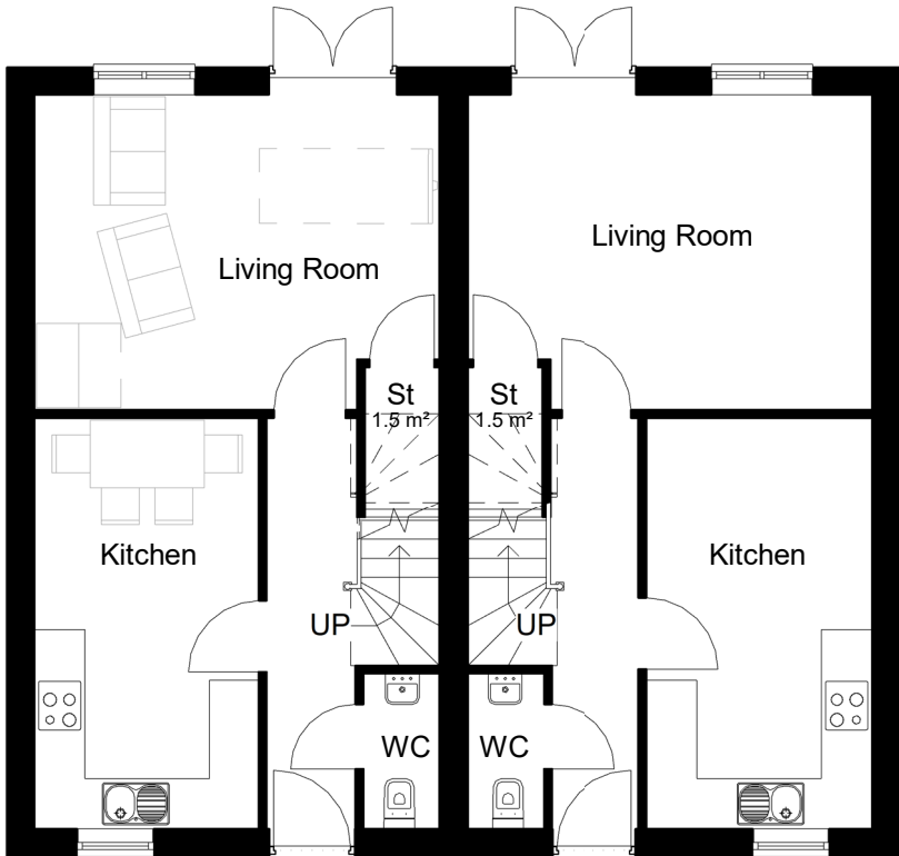
Level 00-Ground Floor Plots 304-305, 372-373 1 : 100
