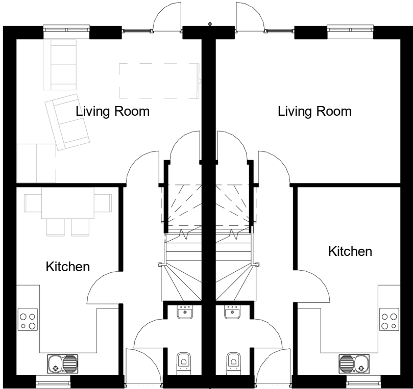
Level 00-Ground Floor Plots 87-90, 98-101, 104-105, 113-114 1 : 100
