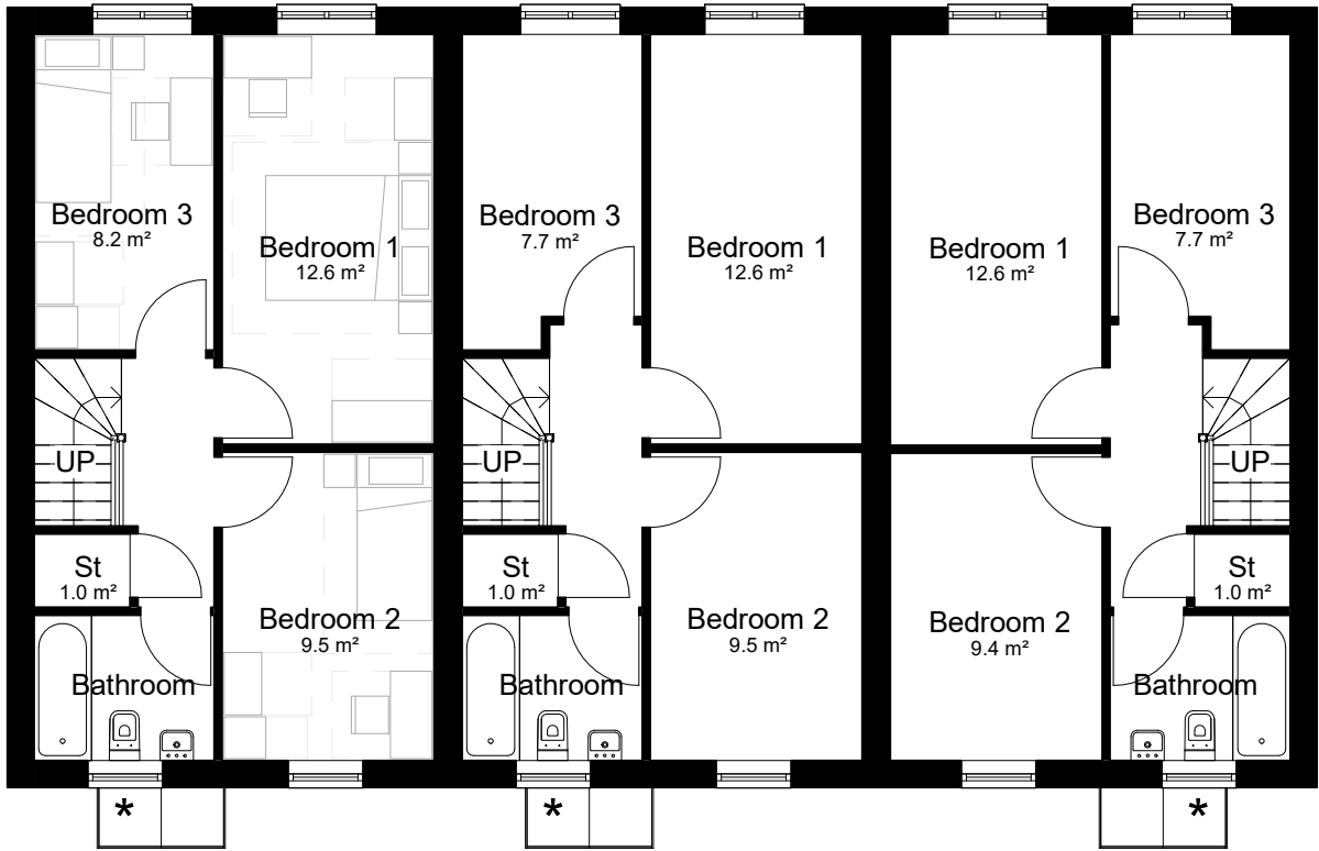
Level 01-First Floor (293-295) 1 : 100
