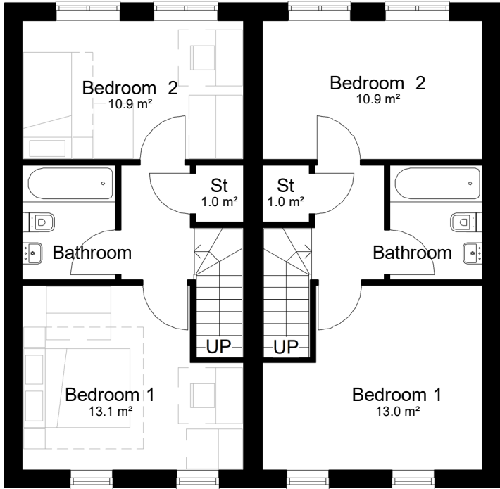
Level 01-First Floor 1 : 100
