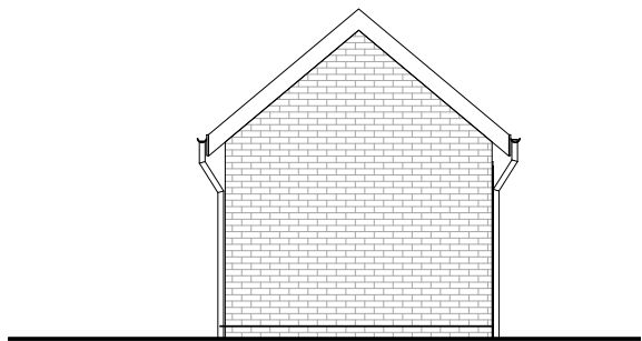
Side Elevation B 1 : 100
