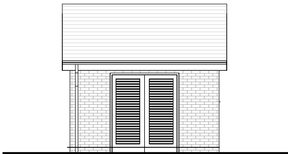
Front Elevation 1 : 100
