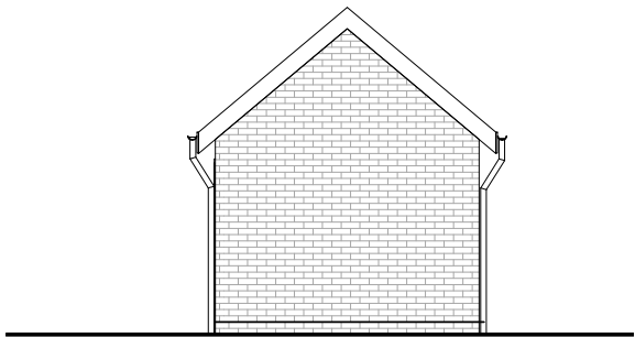
Side Elevation A 1 : 100
