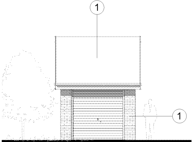
Front Elevation 1 : 100
