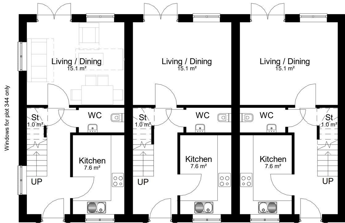
Level 00-Ground Floor 1 : 100
