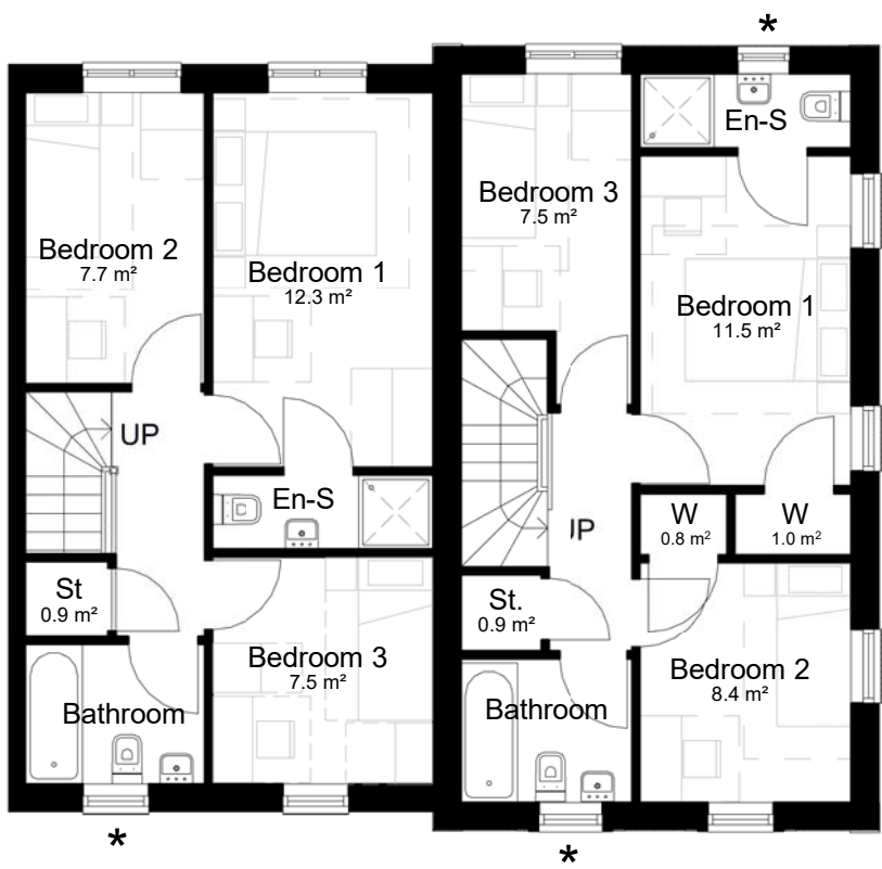
Level 01-First Floor 1 : 100
