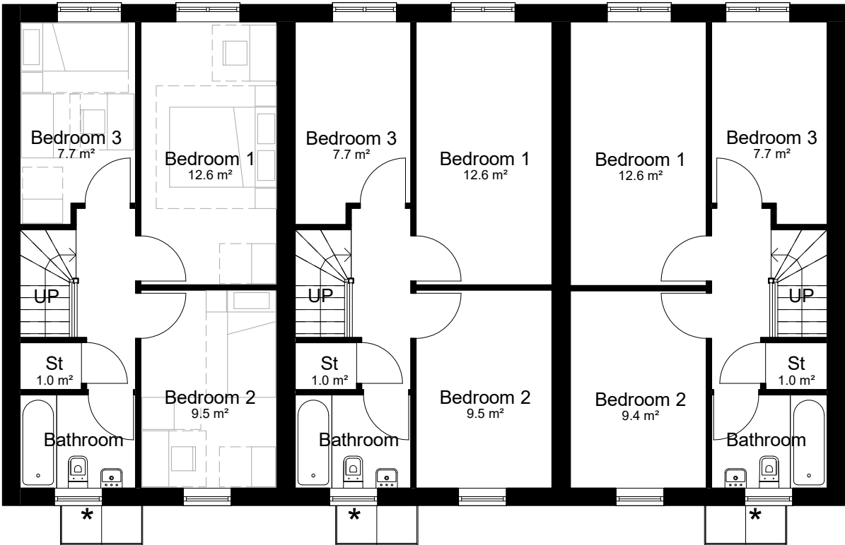
Level 01-First Floor (Plots 331-333) 1 : 100
