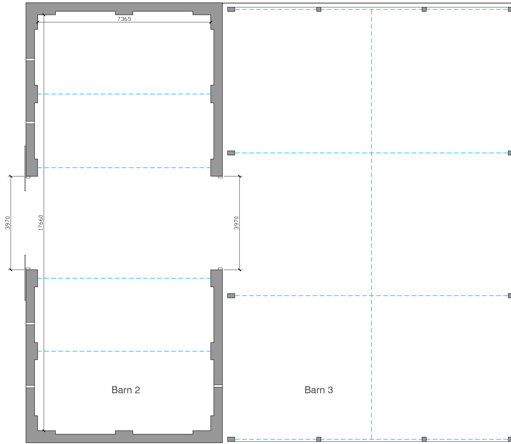
Existing Ground Floor Plan Barn 2 & 3
