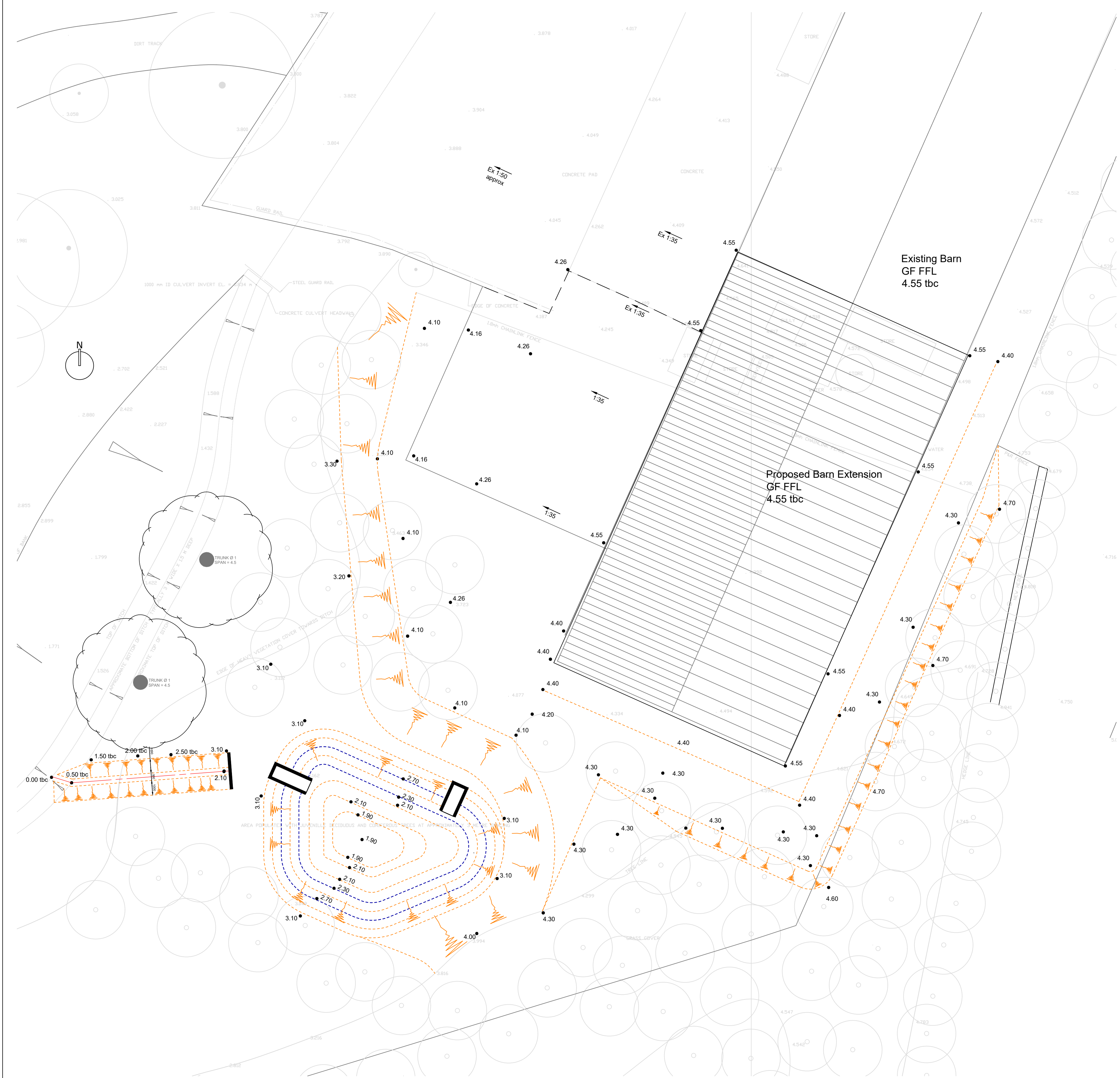
External Levels (1:150)
