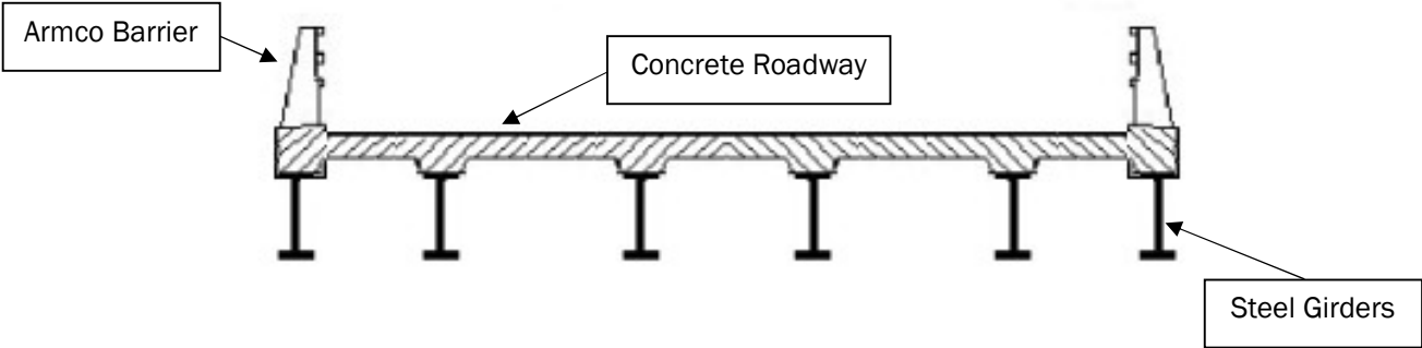
Bridge Cross Section
