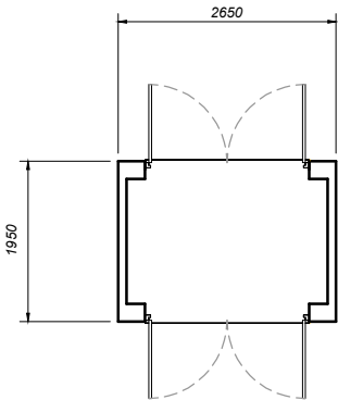
Floor Plan
