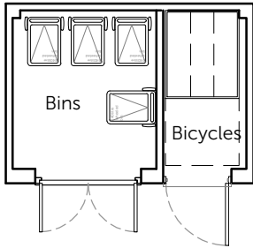
Floor Plan
