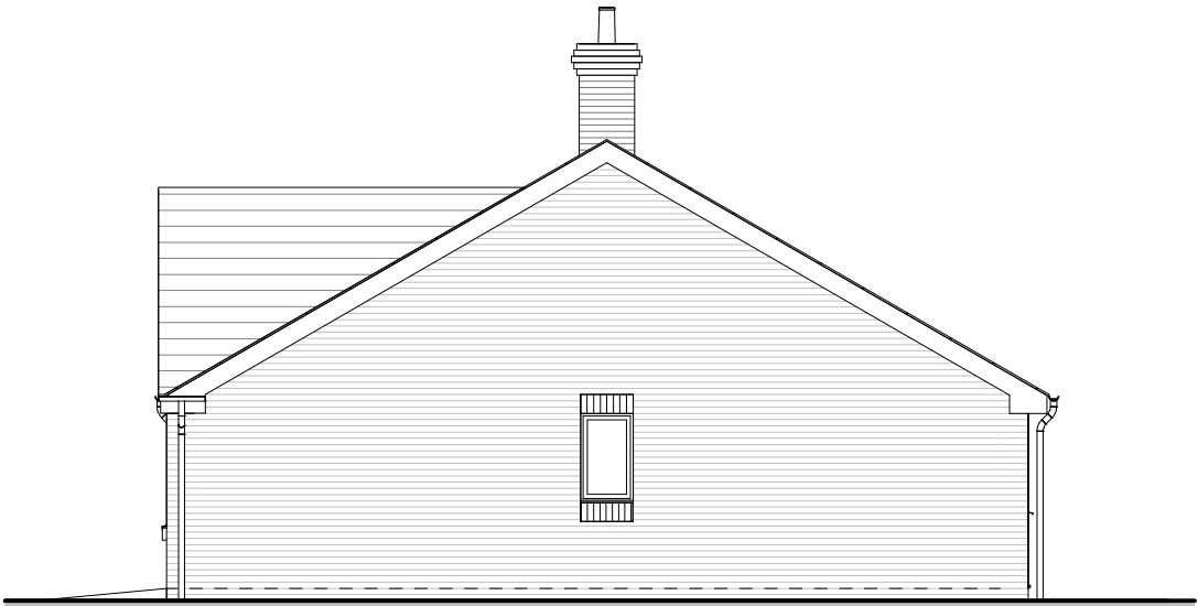
Side Right Elevation
