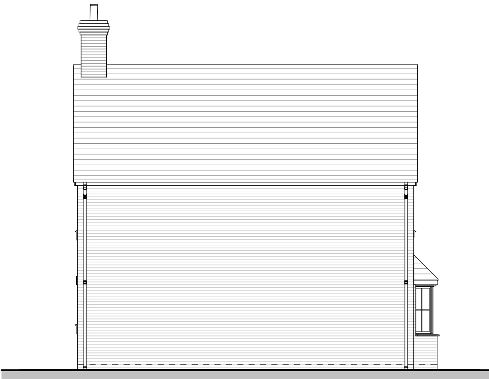
Rear Elevation
