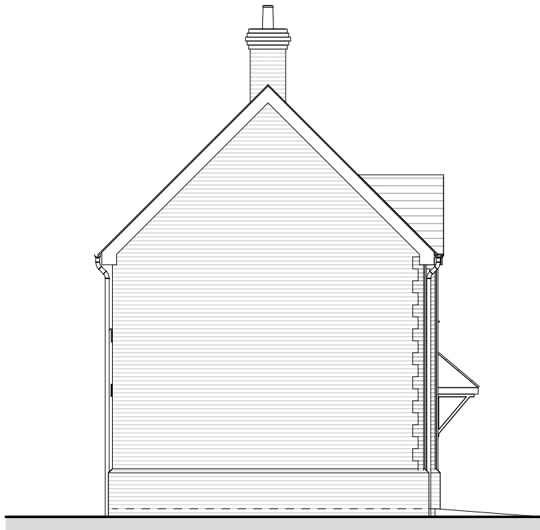
Side Left Elevation
