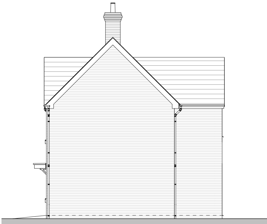
Side Right Elevation
