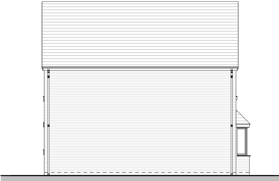
Rear Elevation
