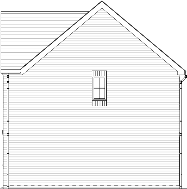
Side Right Elevation
