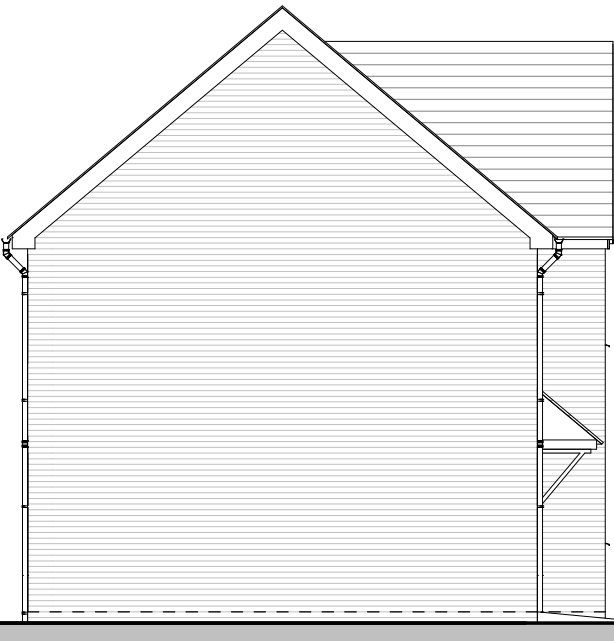
Side Left Elevation
