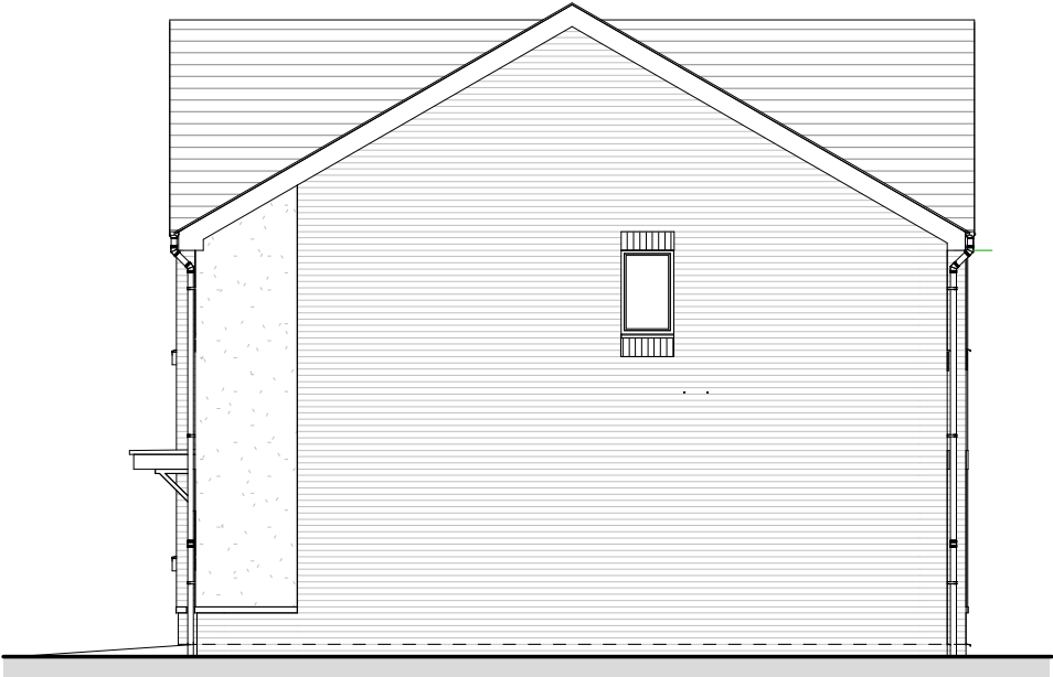
Side Right Elevation
