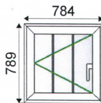
1 - 784w x 789h (Basic Frame Size) Plus 30mm Cill Viewed Outside
