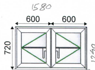
1 - 1200w x 720h (Basic Frame Size) Plus 30mm Cill Viewed Outside
