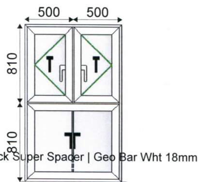
1 - 1000w x 1620h (Basic Frame Size) Plus 30mm Cill Viewed Outside
