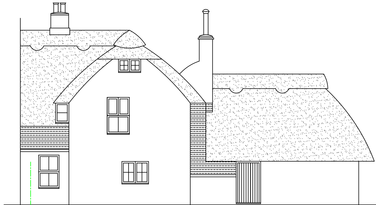
Existing Front Elevation (North)
