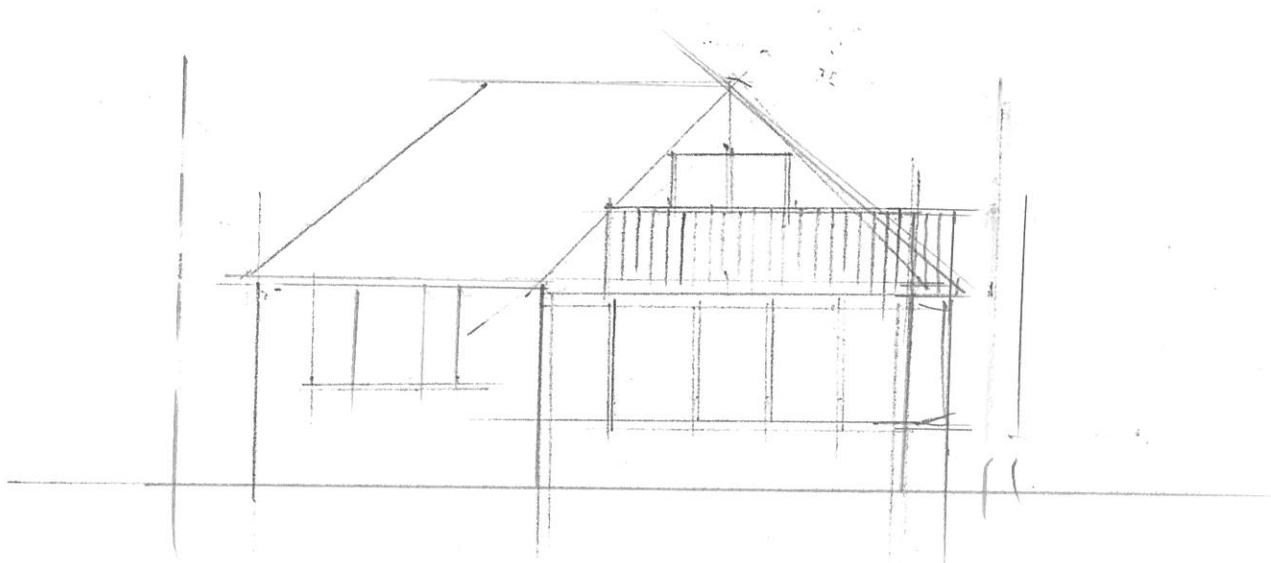
WEST ELEVATION
