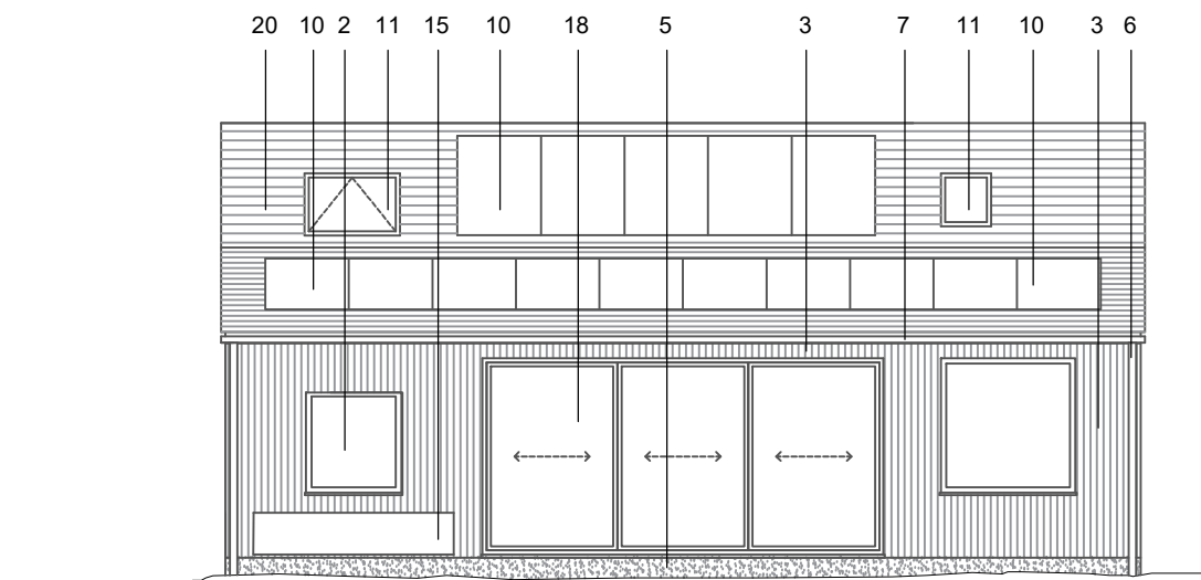
South Elevation
