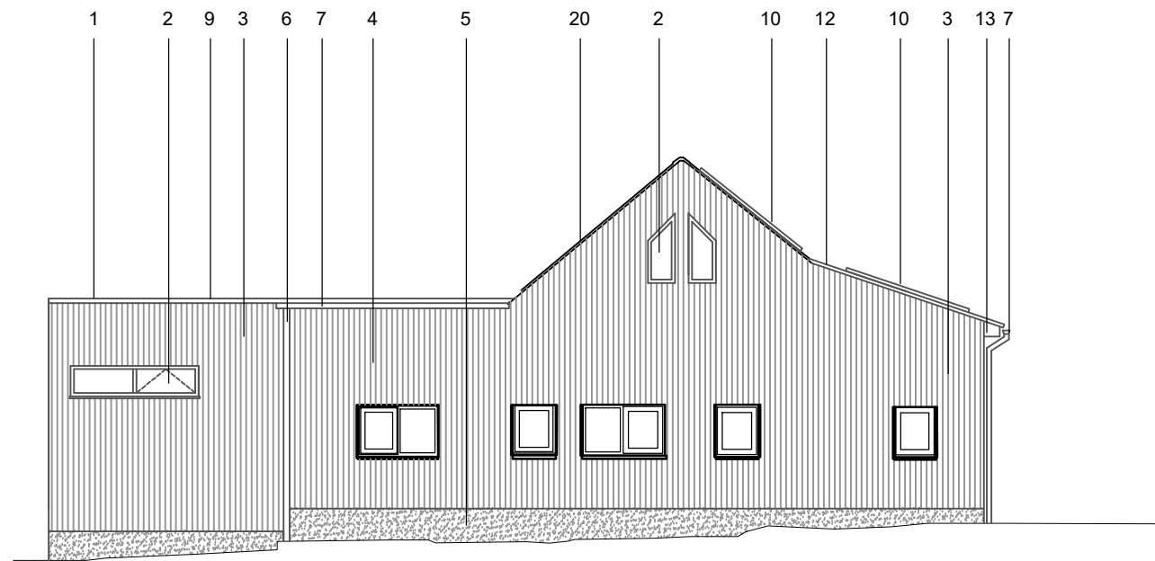
West Elevation
