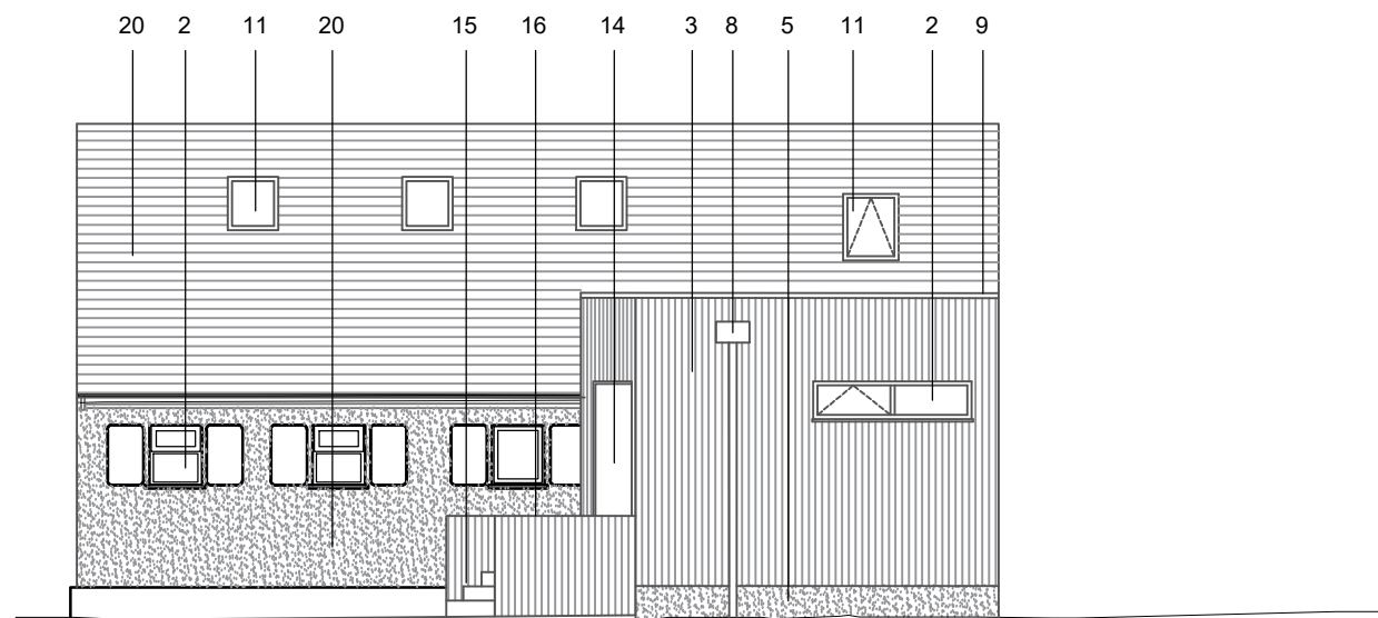
North Elevation
