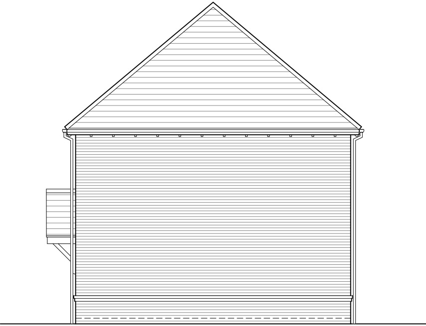
Rear Elevation
