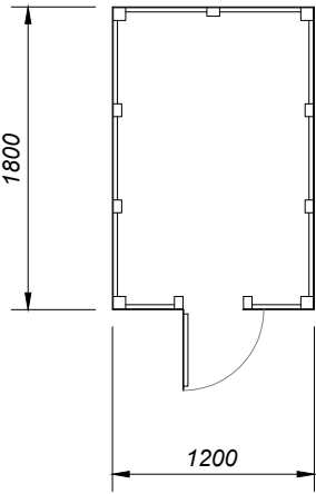
Floor Plan
