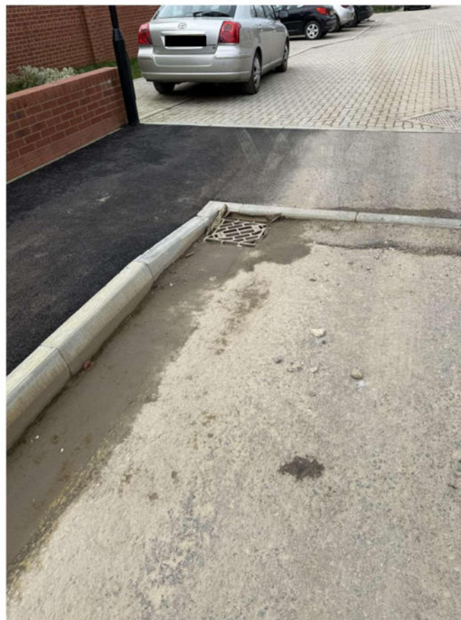
Figure 8 – Road gullies outside Plot 35
