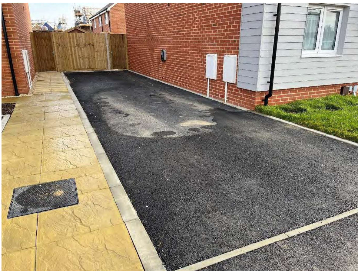
Figure 5 - Plot 296 drive with on-plot drainage installed in line with design drawings
