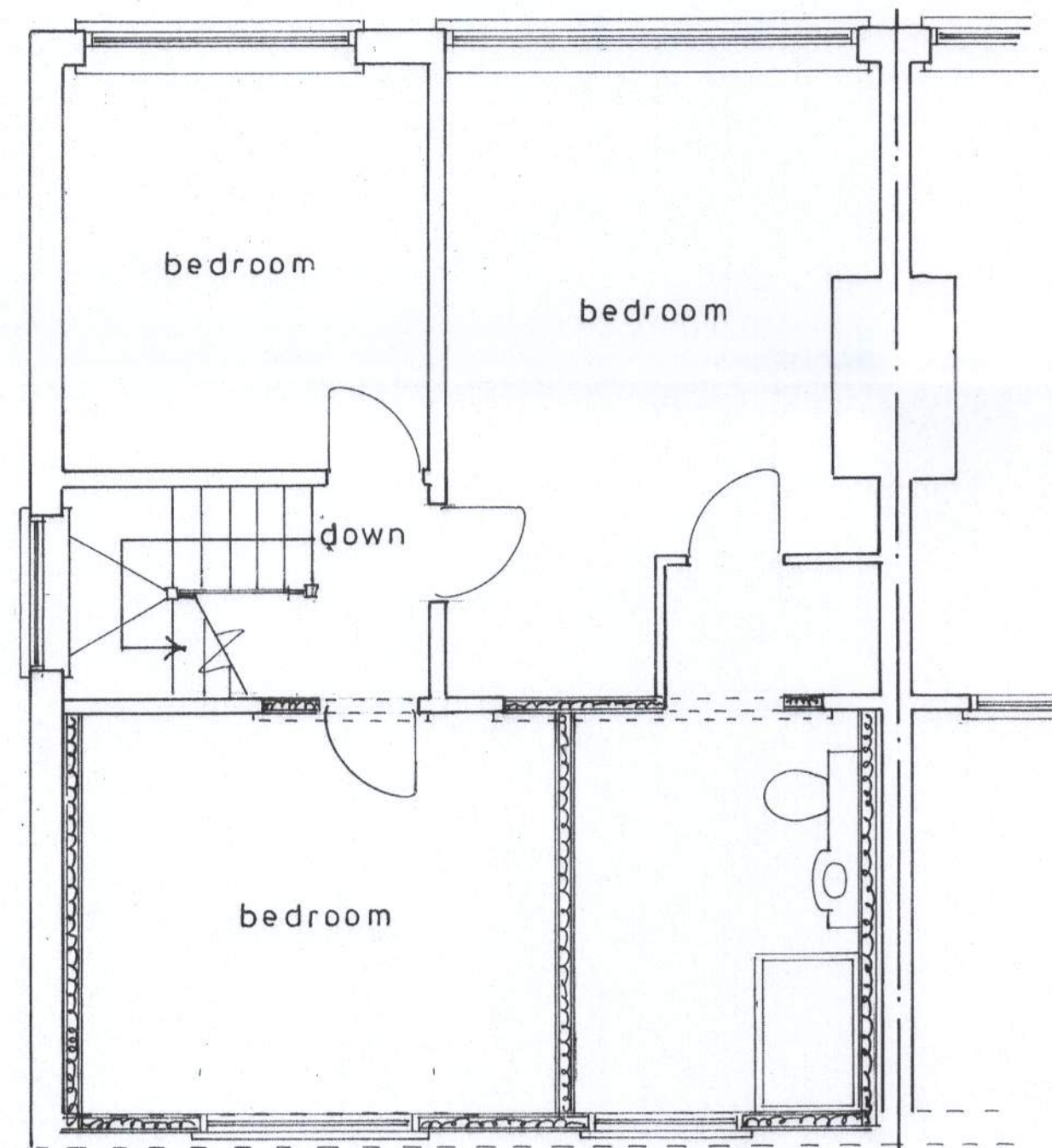
1st floor plan 1 : 50
