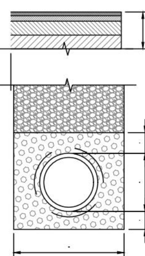
GRANULAR BED AND SURROUND CLASS 'S'
