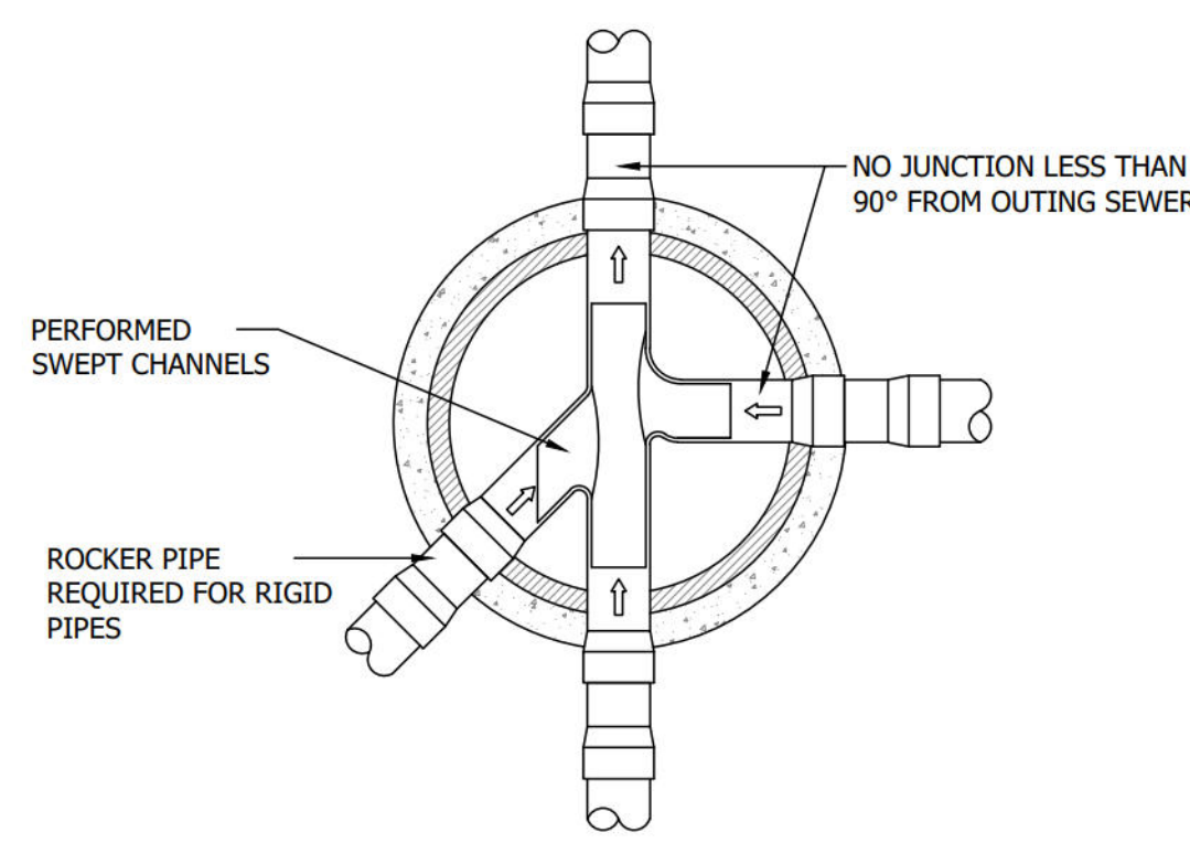
FIGURE B.14 TYPICAL ARRANGEMENT OF PIPE JUNCTIONS WITH MANHOLES
