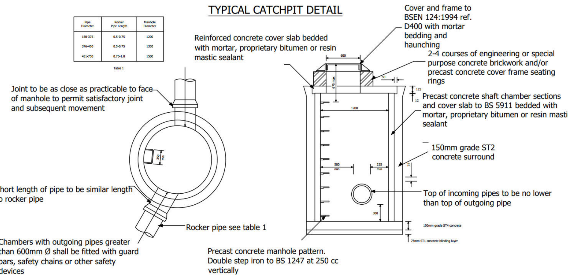
TYPICAL CATCHPIT DETAIL
