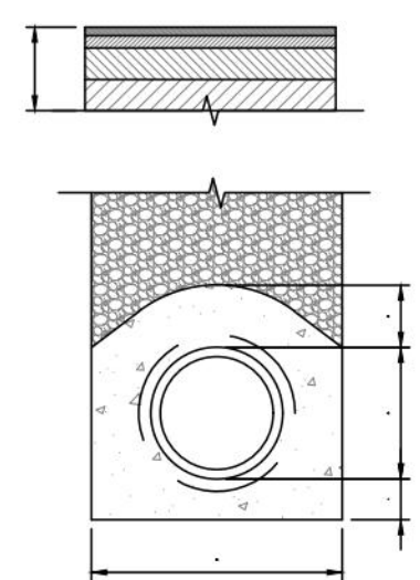
CONCRETE BED AND SURROUND CLASS 'Z'
