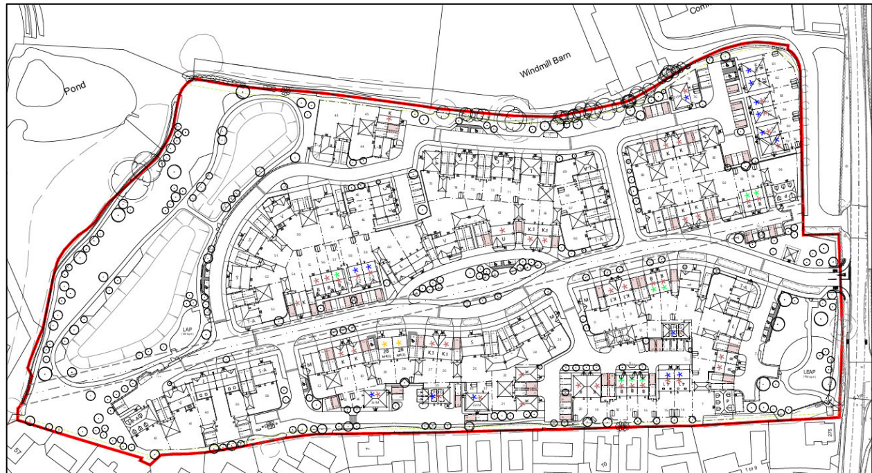
Figure 3.1: Proposed Layout
