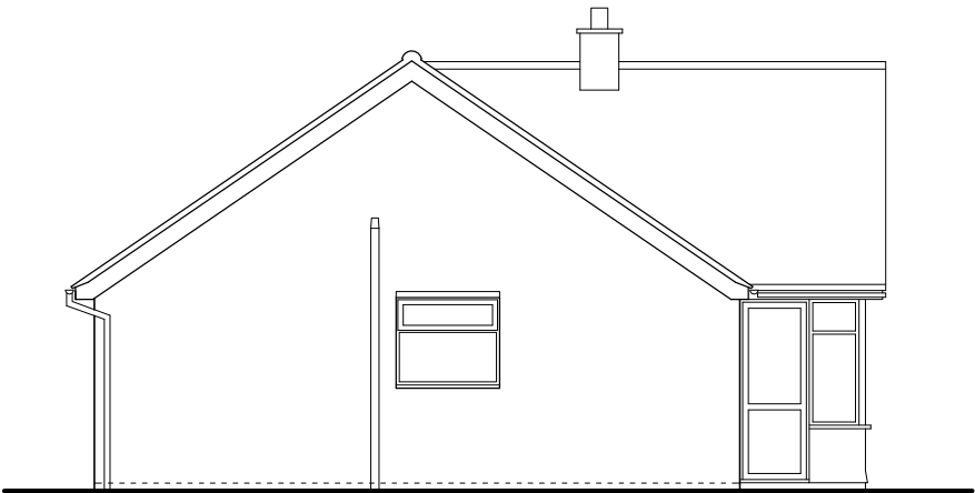
South Elevation
