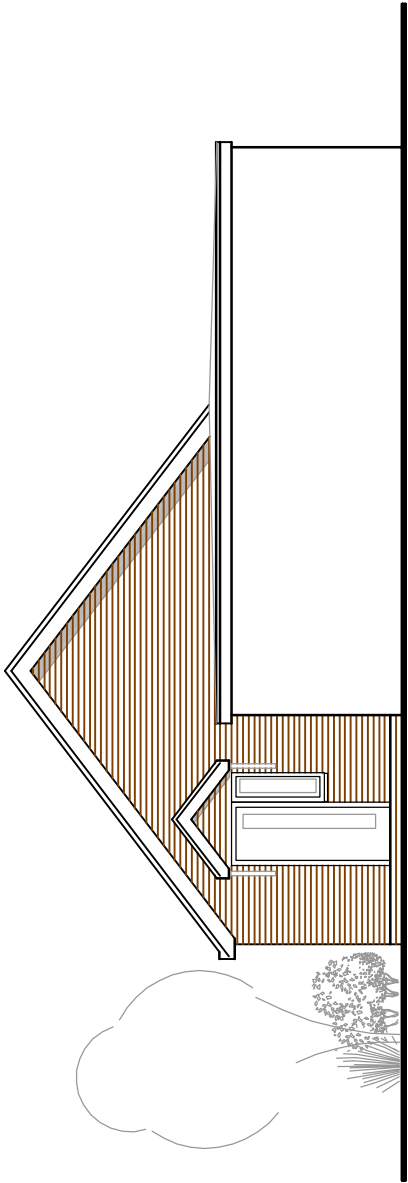
PROPOSED SOUTH ELEVATION 1:100
